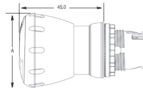
Illuminated and Non-Illuminated Twist-to-Release Operators 30mm, 40mm, and 60mm (D7x-MT)
