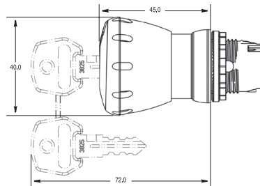
Mushroom Key Release Operator 40mm (D7x-MK)
