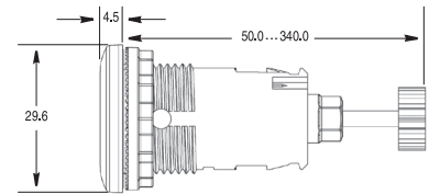
Reset Operators (D7x-R)
