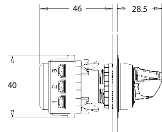
Potentiometer with Resistive Element (D7P- POT)
