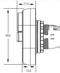
Illuminated and Non-Illuminated 2-Position Multi-Function Operators (D7x-LU2 & D7x-U2)
