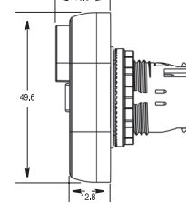
Toggle Switch Operators (D7x-JM)
